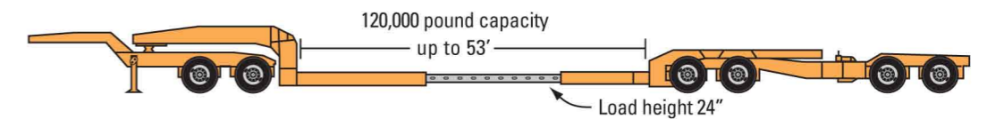
Multiple Axle High Tonnage Double Drop
