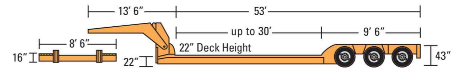
Removeable Gooseneck
