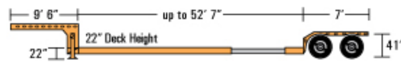
Double Drop Stretch
