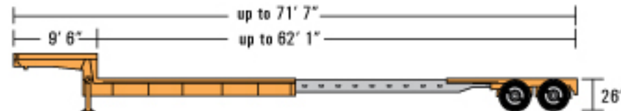
Low Profile Stepdeck Stretch
