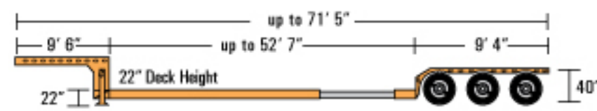
3-Axle Double Drop Stretch
