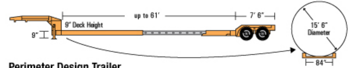
Perimeter Design Trailer
