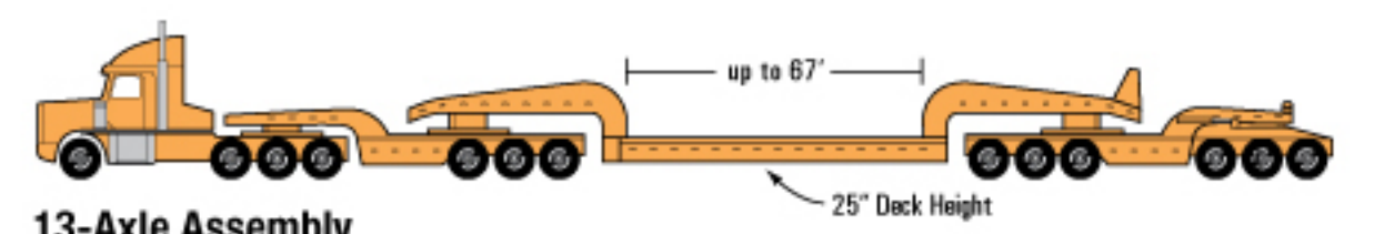
13-Axle Assembly
