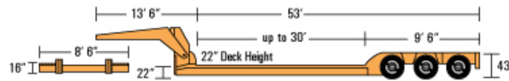
Removeable Gooseneck (RGN)
