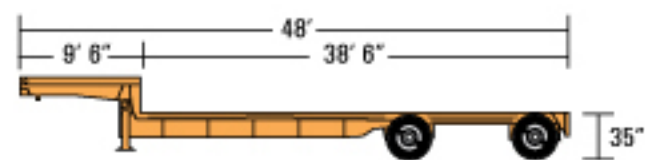
48' Stepdeck
