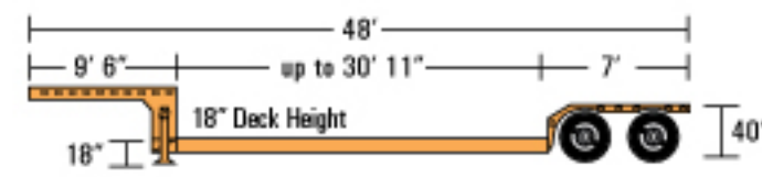
Double Drop
