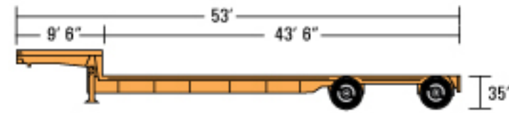
53' Stepdeck
